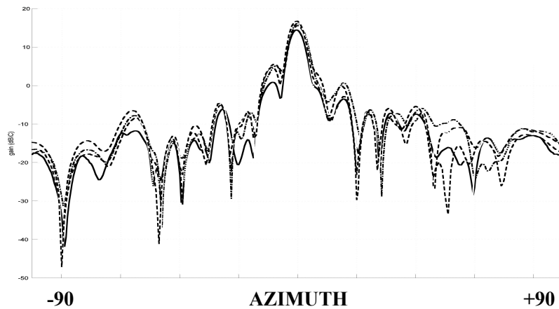
Fig. 5. Gain pattern of S-band array for various blockage levels by the S-band array
