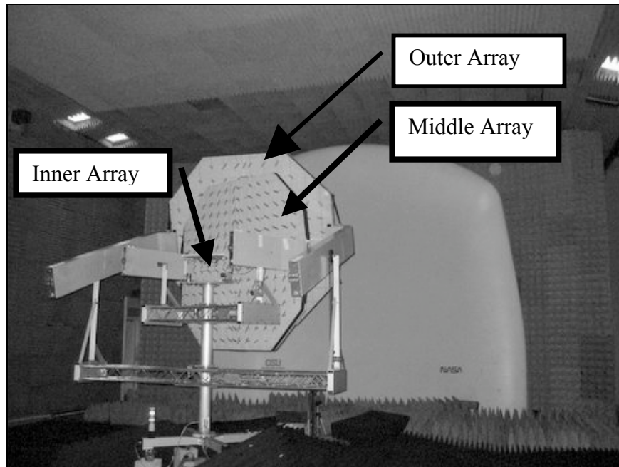
Fig. 1. Photograph of set of 3 mutually transparent arrays (set up for measurement in the Ohio State Univ. Compact Range)
