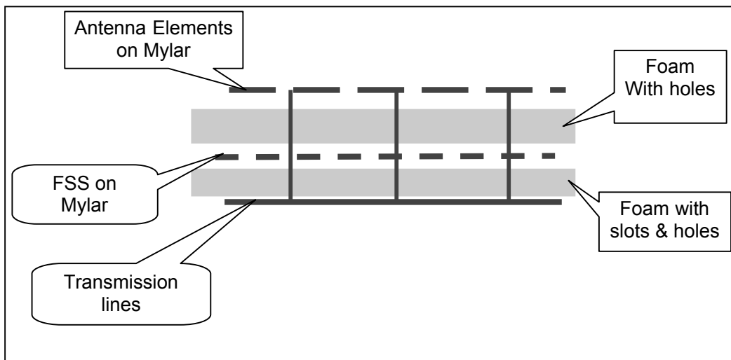
Fig. 2. Side diagram of an individual array
